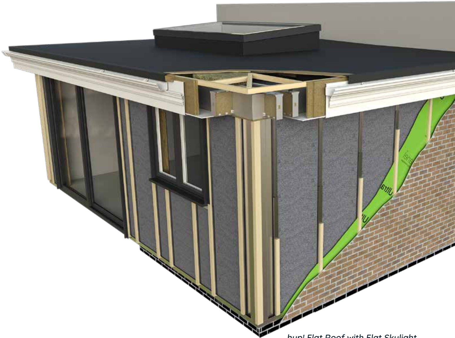
hup! Flat Roof with Flat Skylight.
